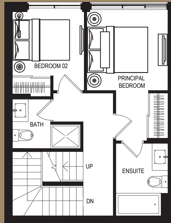
FOURTH FLOOR
